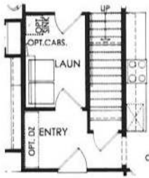
Loft w/ Bedroom and Bath 1st Floor
