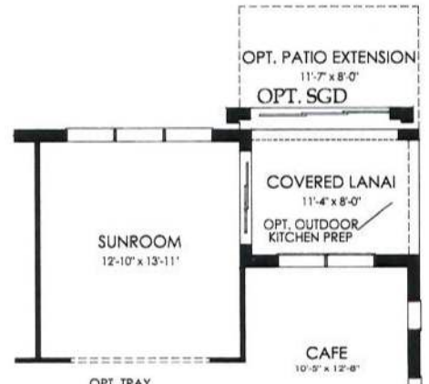
Sunroom Adds 177SF
