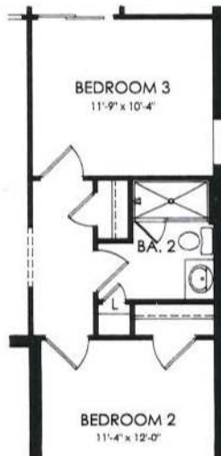
Shower @ Alternate Bath 2
